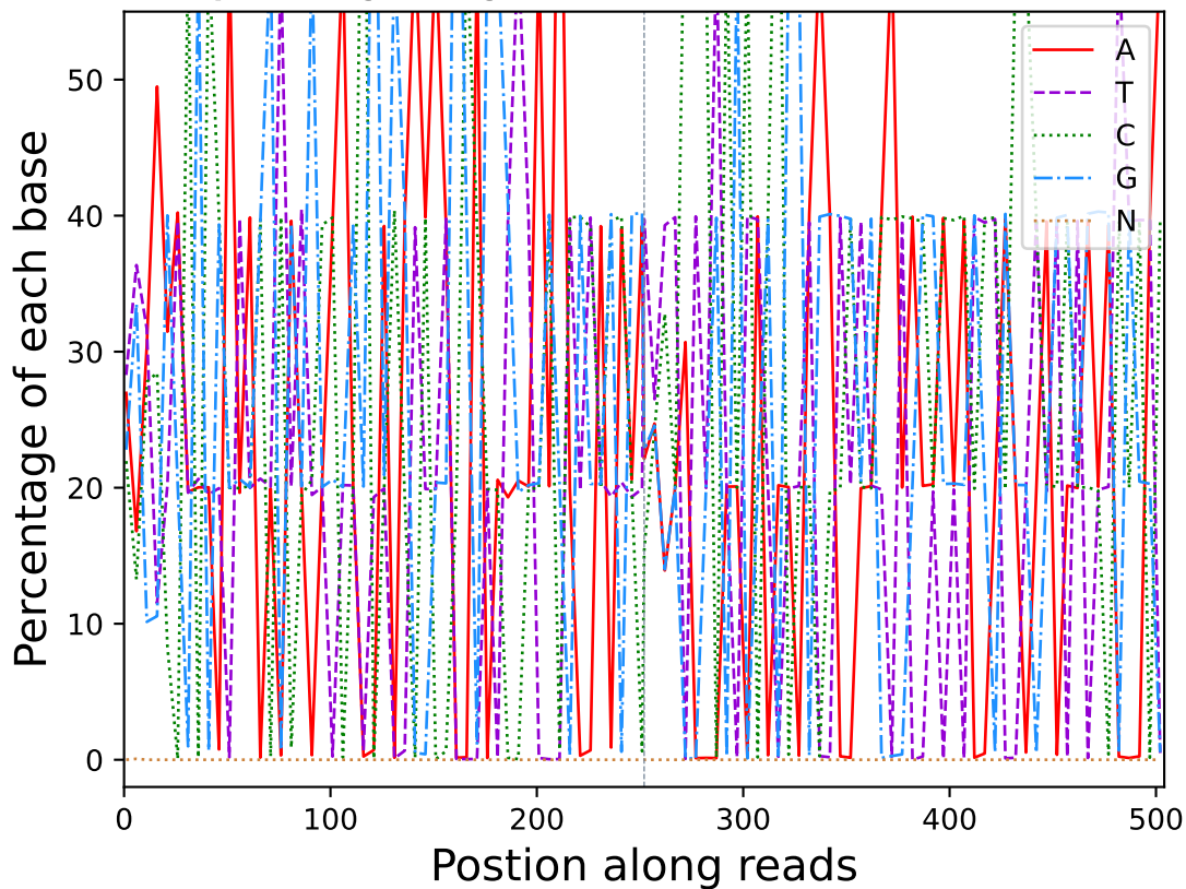
Base percentage along reads (R10121)
